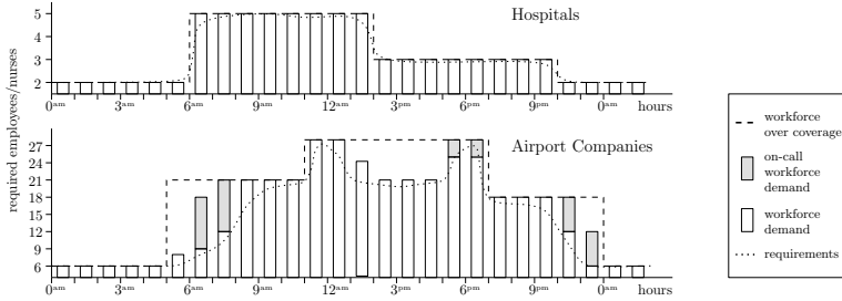
Fig. 1 The coverage function f_C examples
